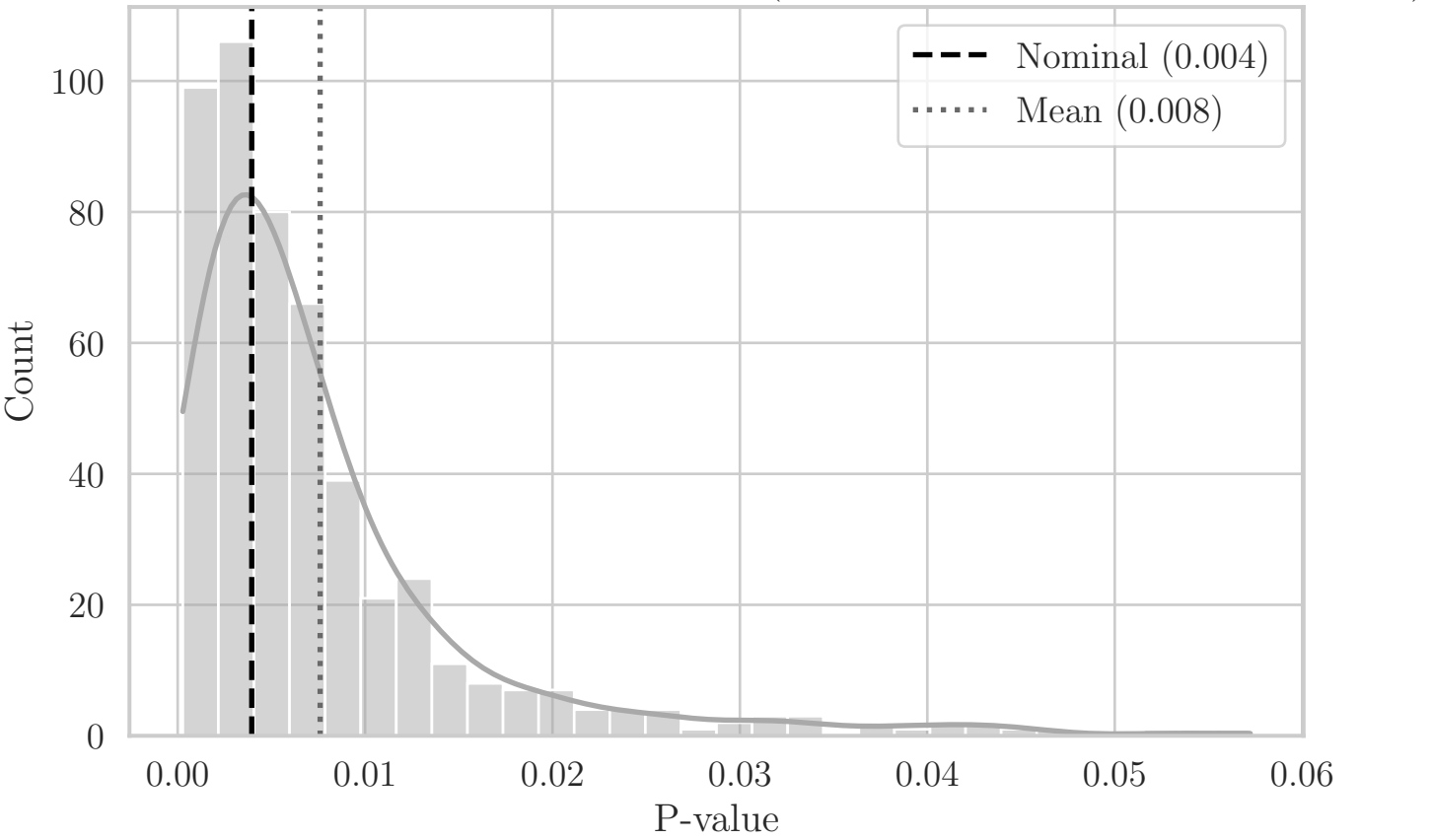
MC Distribution of P-values for T T-Dist (Aggregated Top-Left Quadrant YZ)
