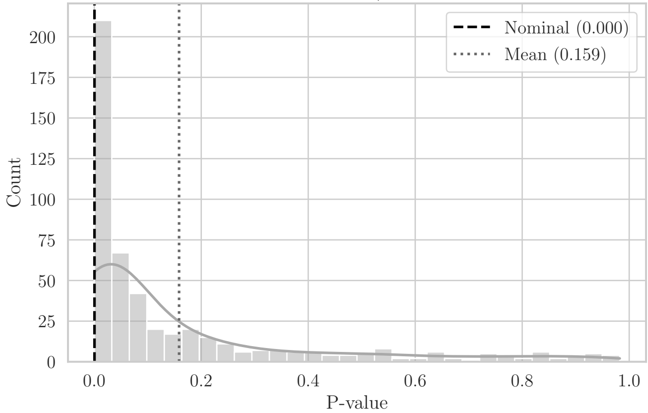
MC Distribution of P-values for ST Area (Aggregated Top-Right Quadrant YZ)
