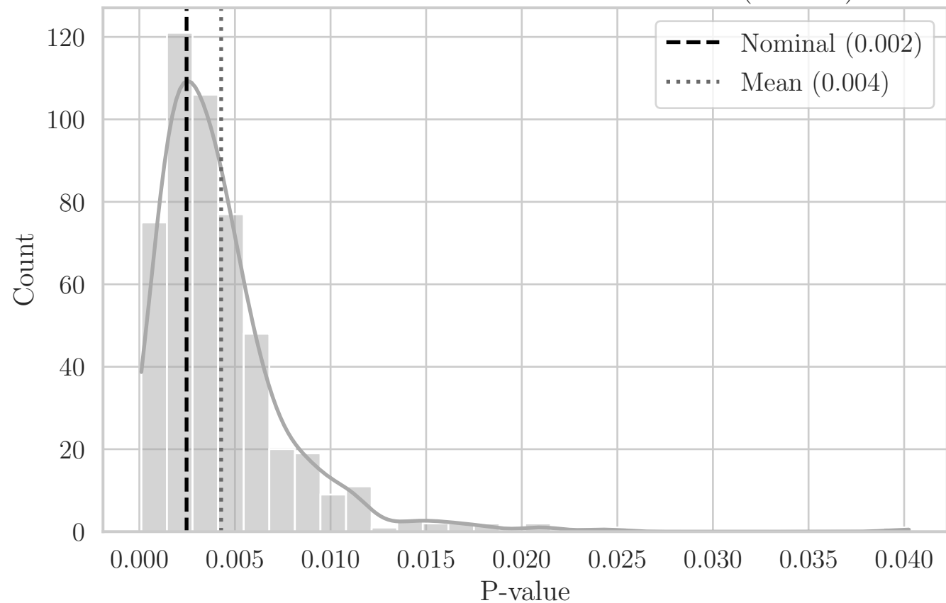
MC Distribution of P-values for T T-Dist (YP YZ)
