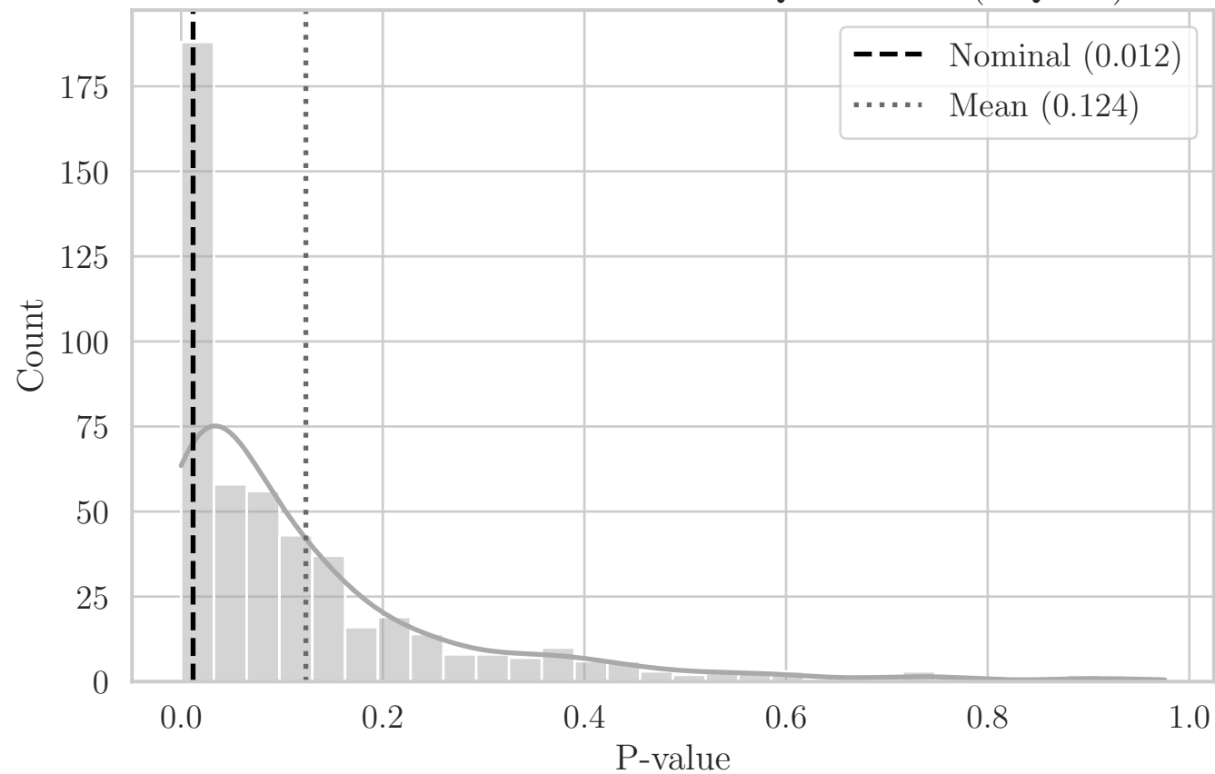
MC Distribution of P-values for QRS T-Dist (YQ XY)
