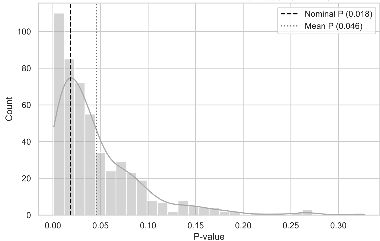
MC Distribution of P-values for QRS Angle (Aggregated XY)
