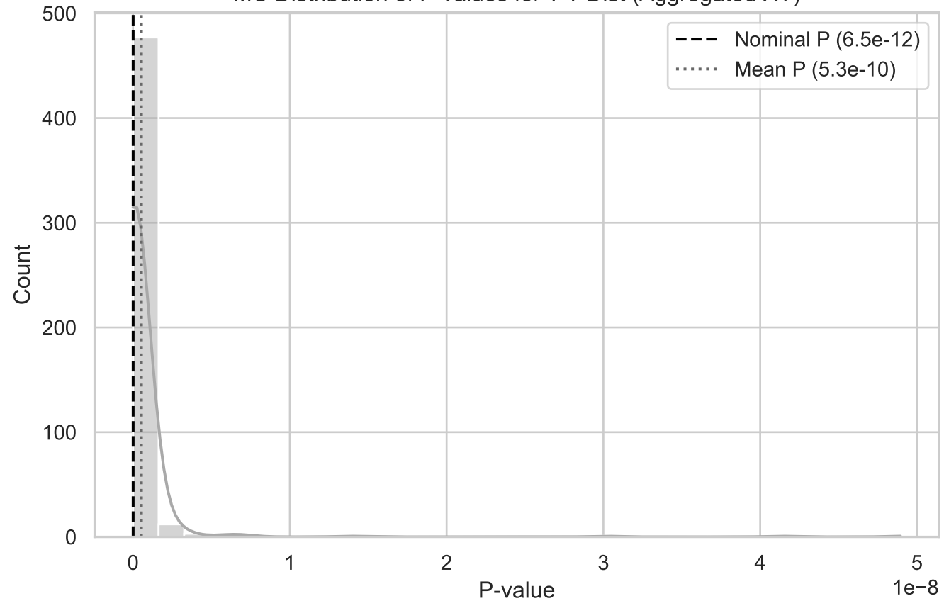
MC Distribution of P-values for T T-Dist (Aggregated XY)
