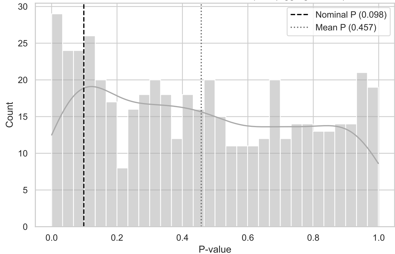
MC Distribution of P-values for ST Compact (Aggregated YZ)
