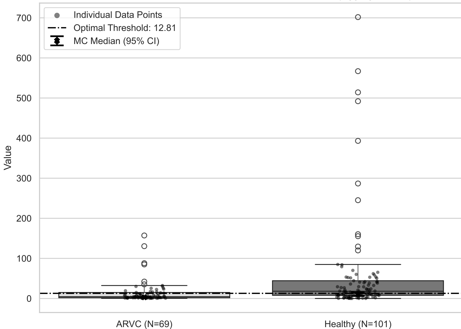
Box Plot of Nominal Data with MC Medians for ST Area (Aggregated XY)
