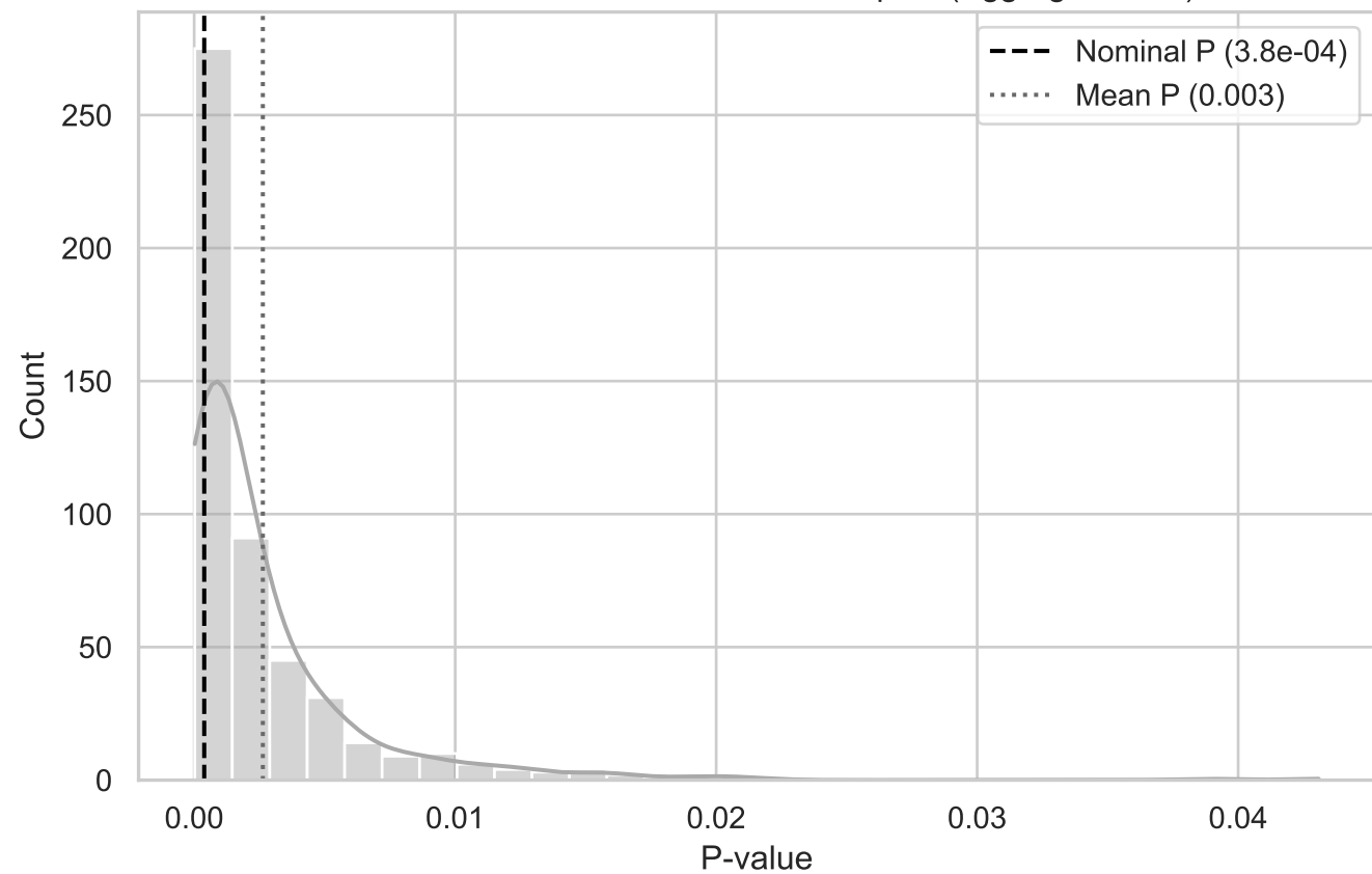
MC Distribution of P-values for T Compact (Aggregated XY)
