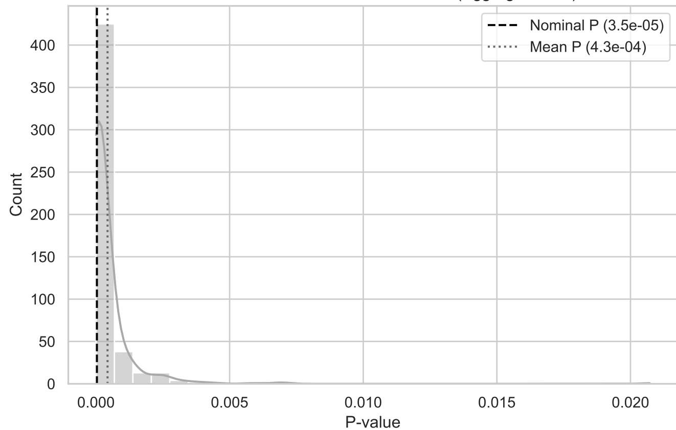
MC Distribution of P-values for T T-Dist (Aggregated YZ)
