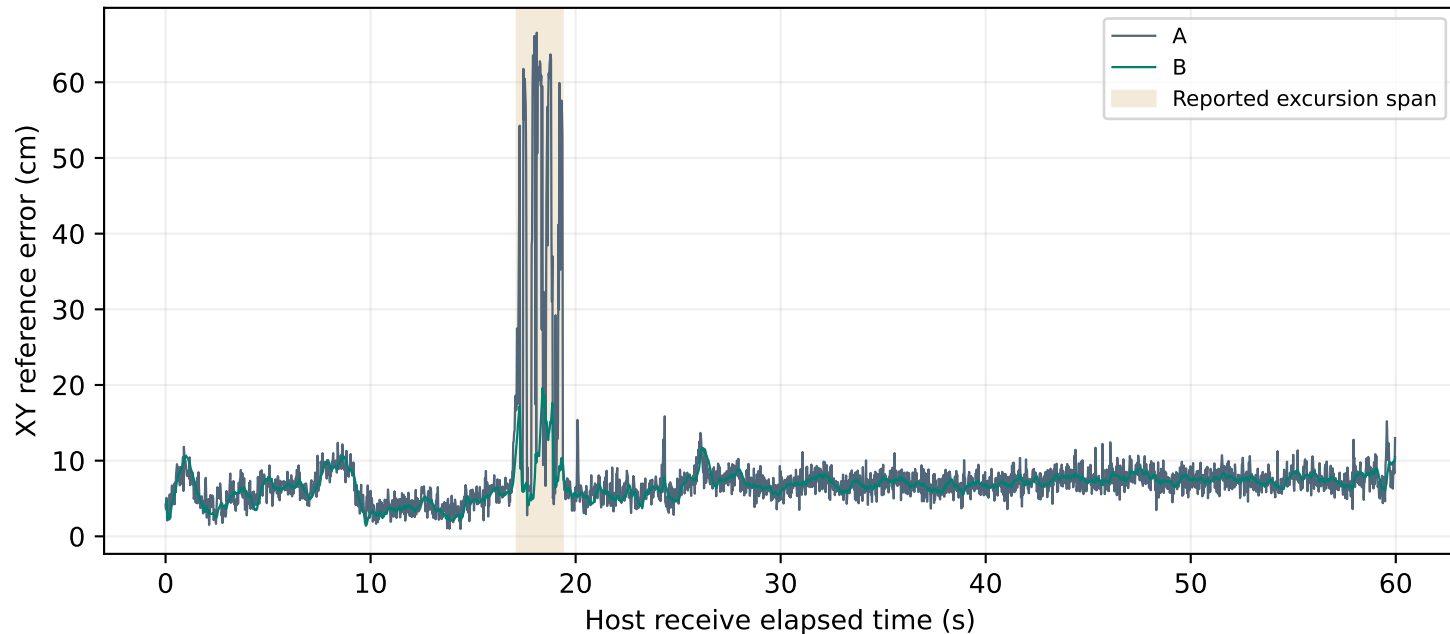
Measured static capture: A vs B (H80)
