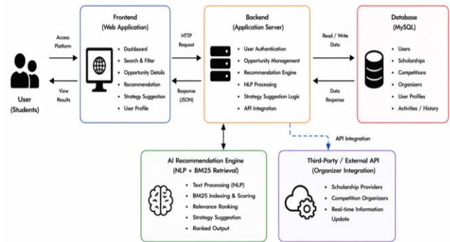
Fig. 1. System Architecture of the Proposed Platform.
