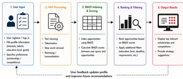
Fig. 2. Recommendation Workflow of the Proposed System.
