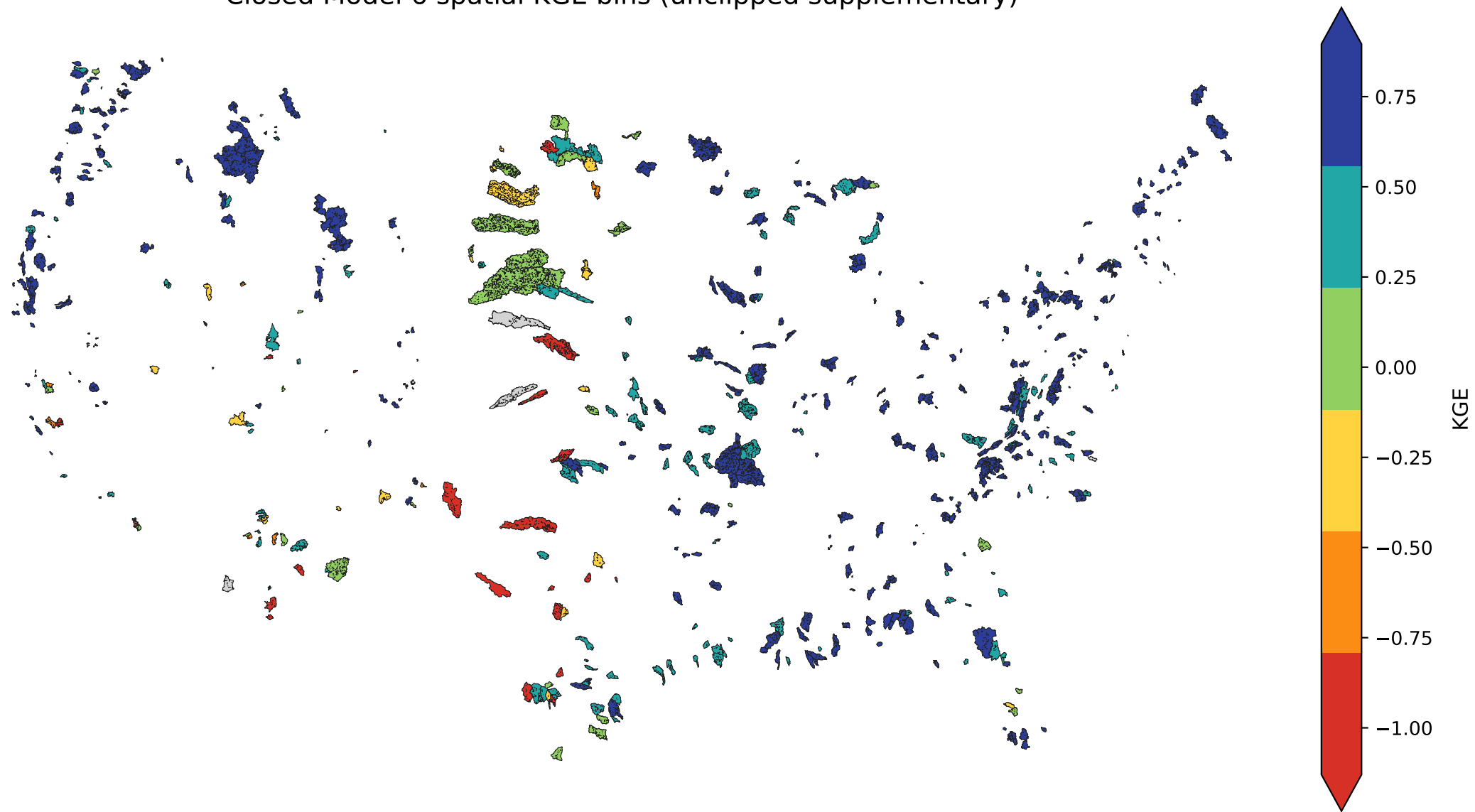
Closed Model 6 spatial KGE bins (unclipped supplementary)
