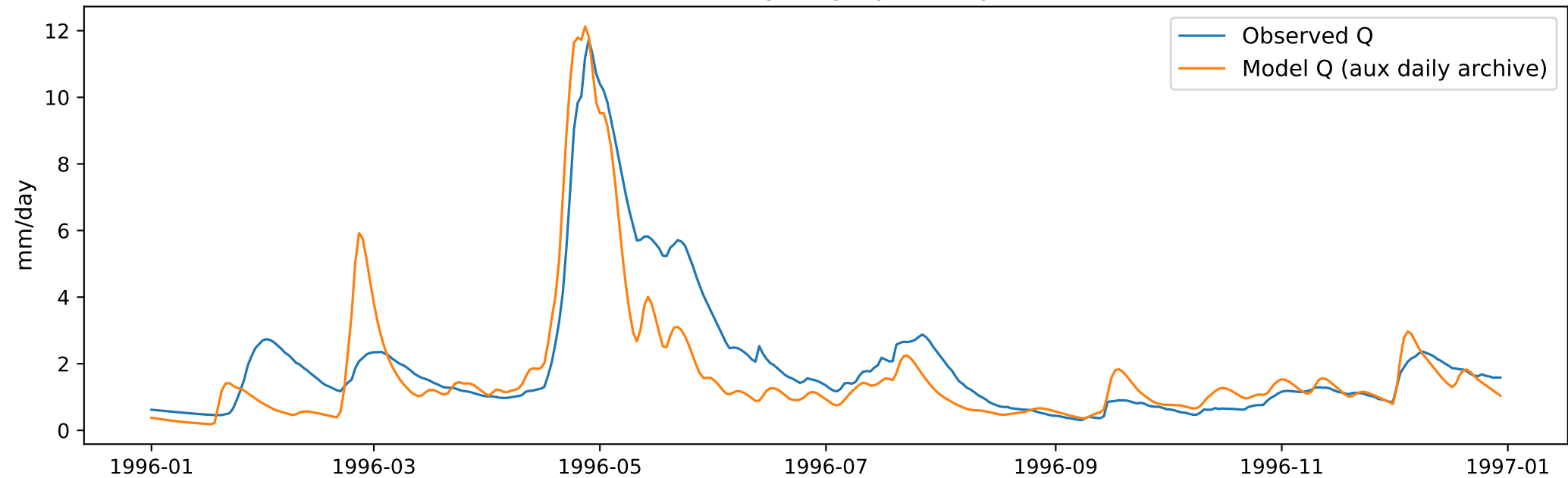
Basin 1013500 hydrograph sample (1996)
