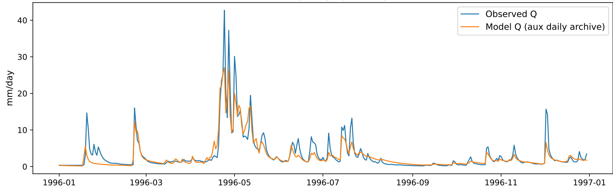
Basin 1052500 hydrograph sample (1996)
