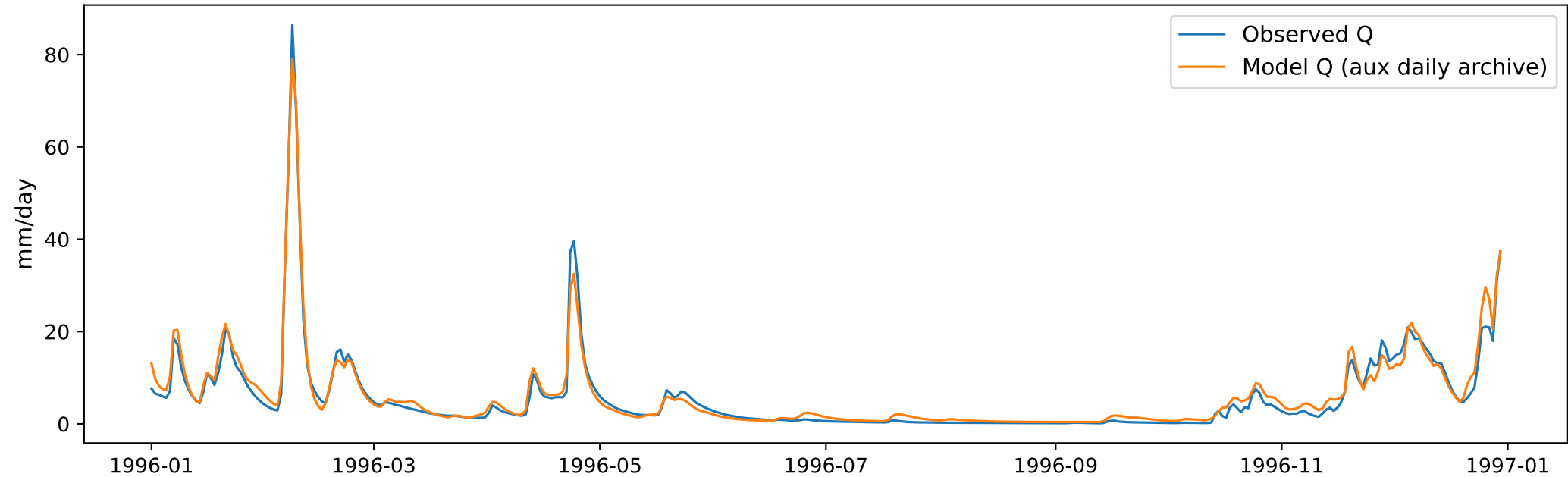
Basin 14301000 hydrograph sample (1996)
