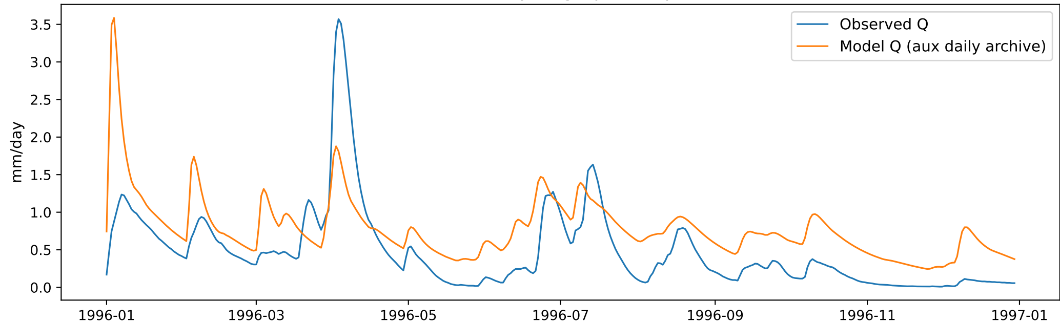
Basin 2310947 hydrograph sample (1996)
