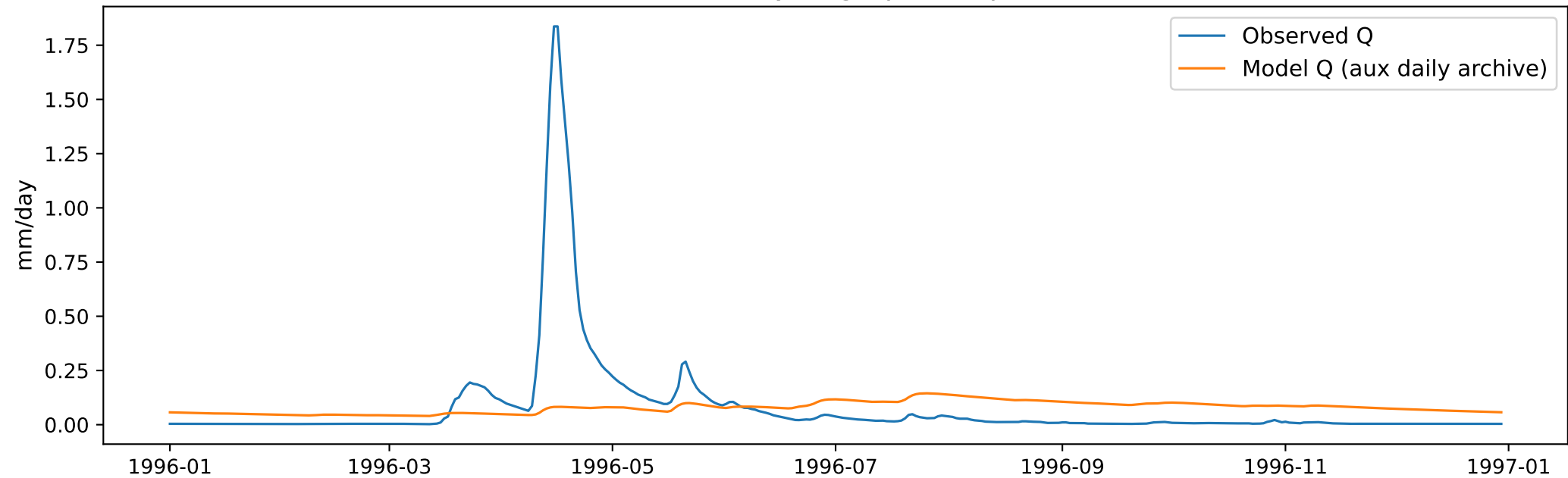
Basin 5056000 hydrograph sample (1996)
