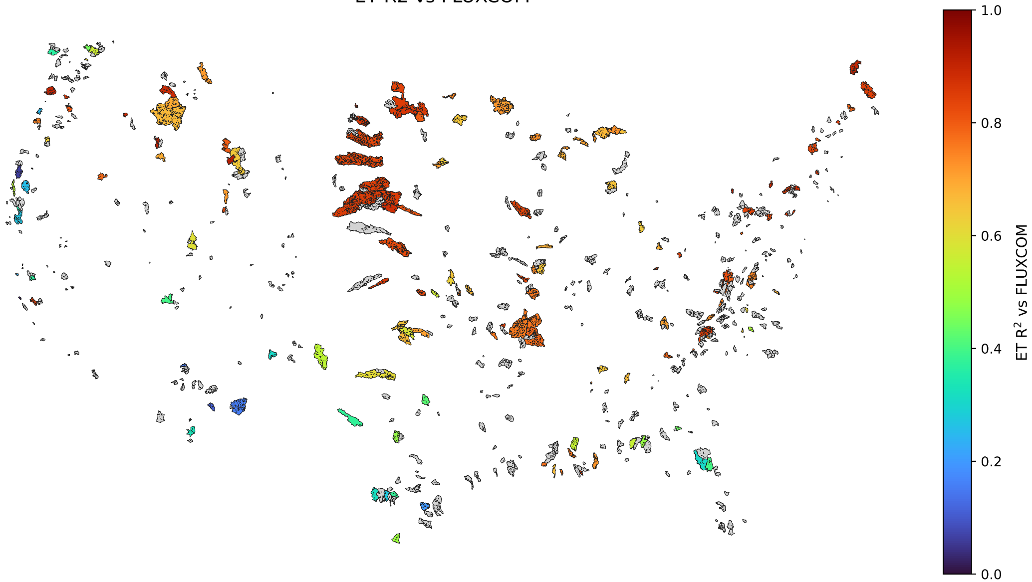
ET R 2 vs FLUXCOM
