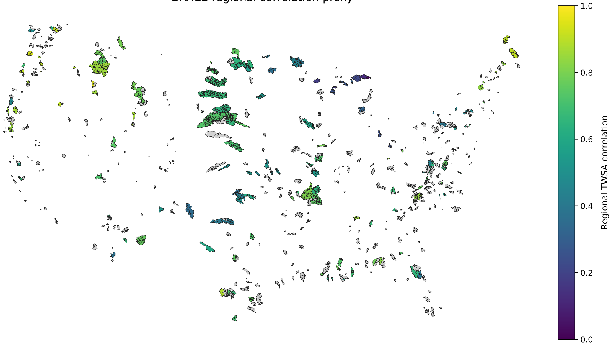
GRACE regional correlation proxy
