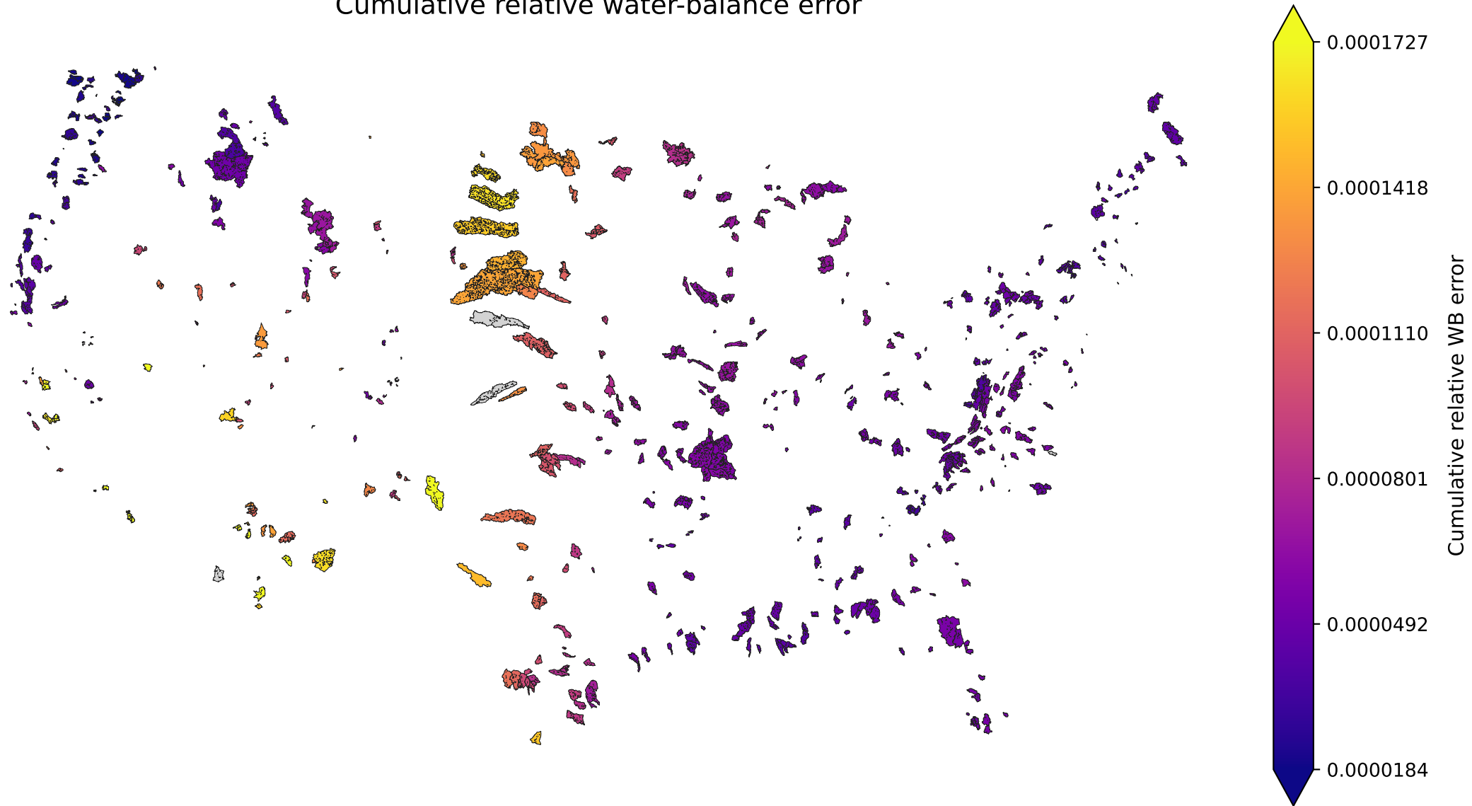
Cumulative relative water-balance error
