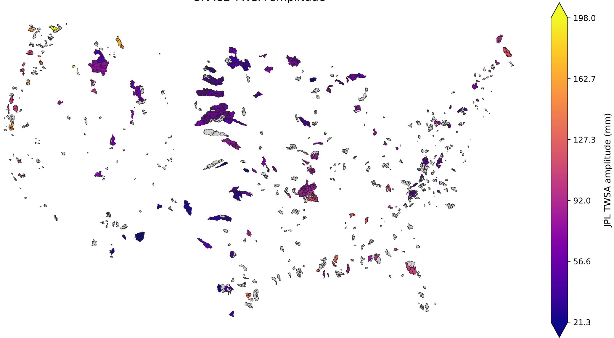
GRACE TWSA amplitude
