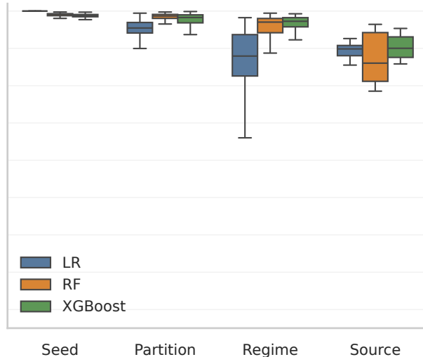
Rank Spearman
