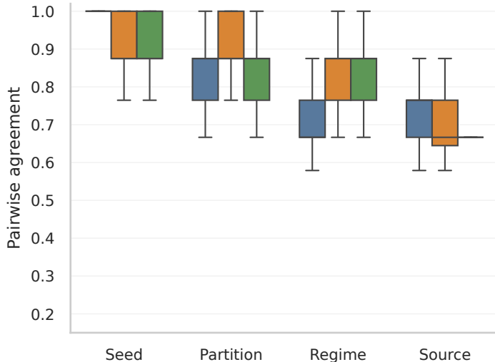
Top-15 Jaccard
