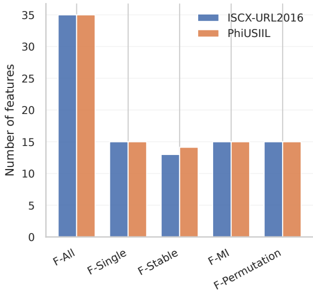
Retained features
