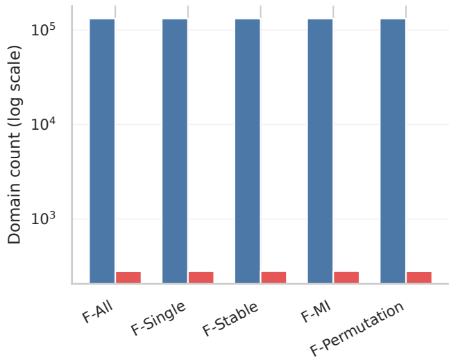
Distinct domains among false positives
