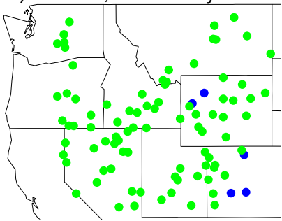
D) RCP8.5, midcentury
