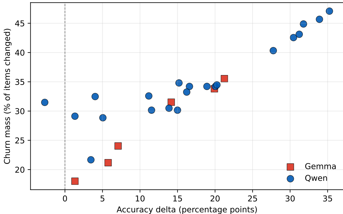
Accuracy gains can coincide with item-level churn
