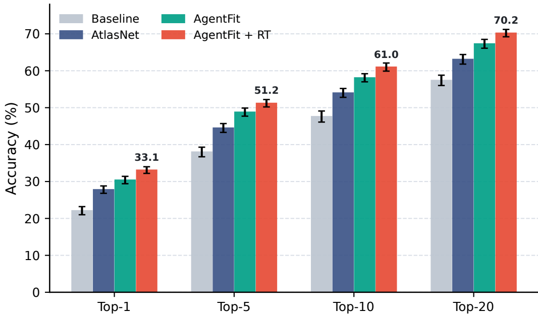
Cross-modal Retrieval Benchmark
