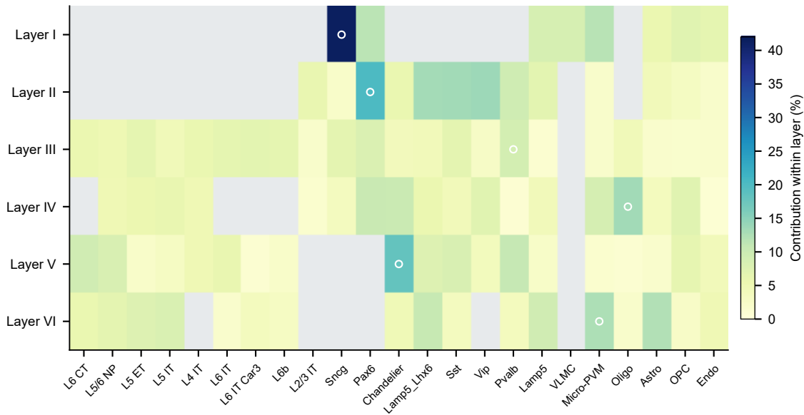
Cell-type contributions differ across cortical layers
