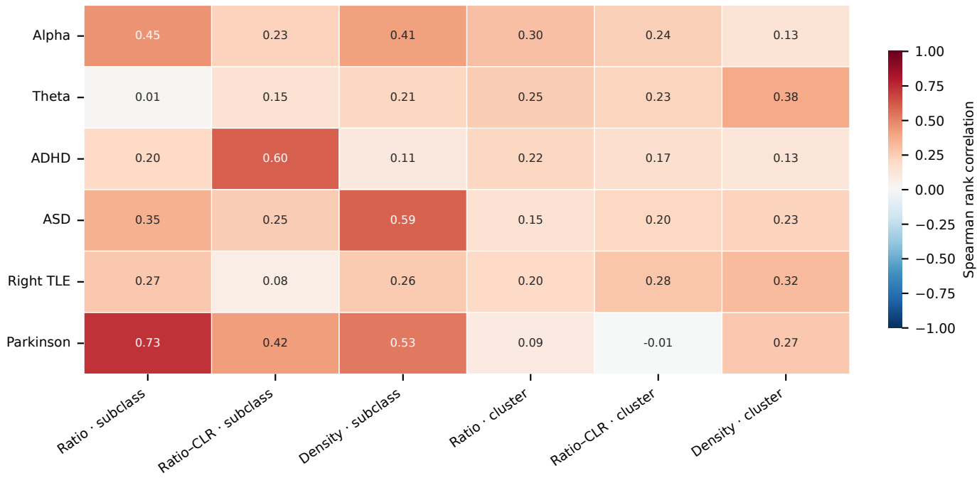
Agreement between held-out SHAP and dominance rankings
