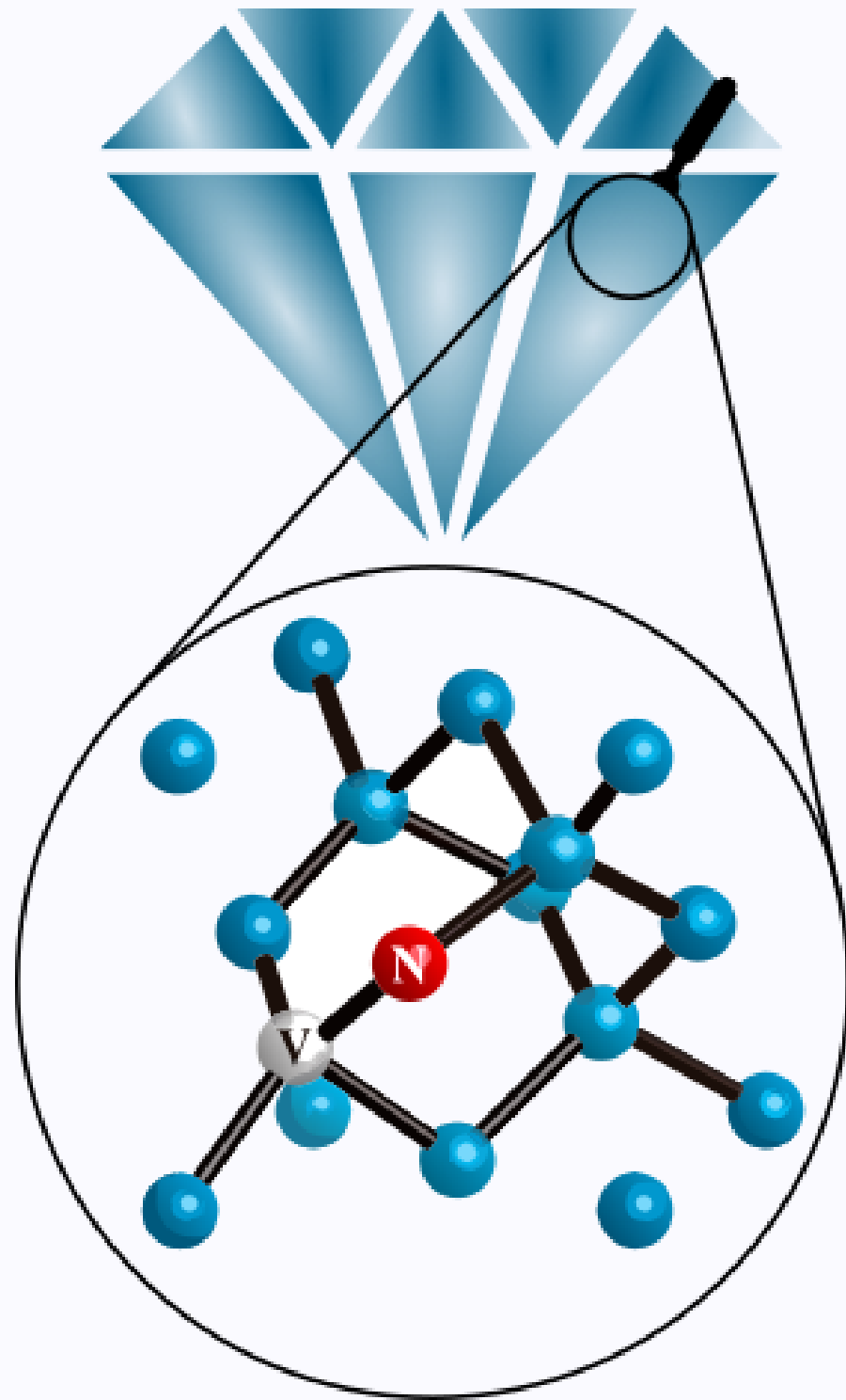
Nitrogen-Vacancy center
