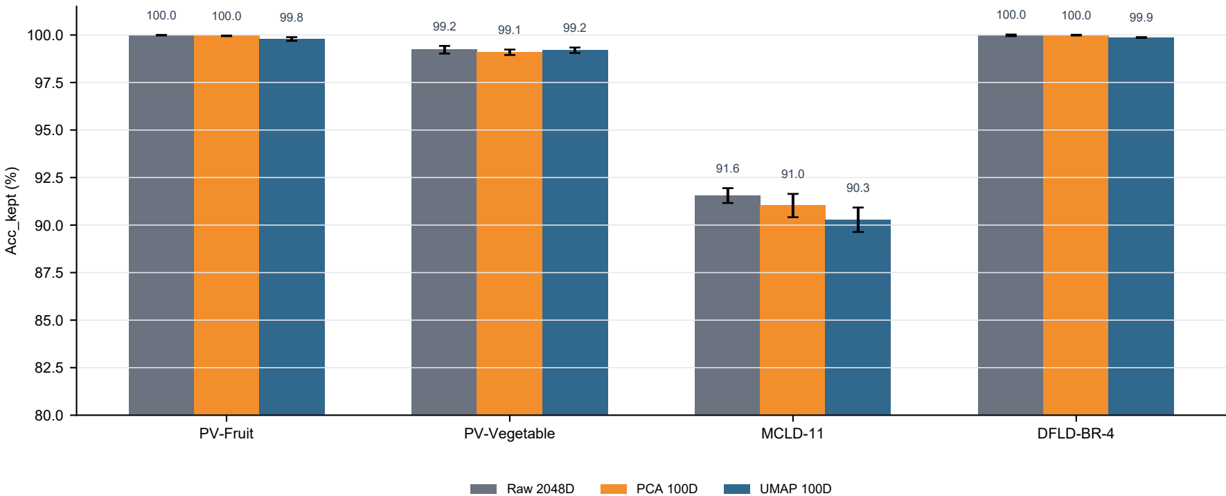
Fair Raw/PCA/UMAP comparison
