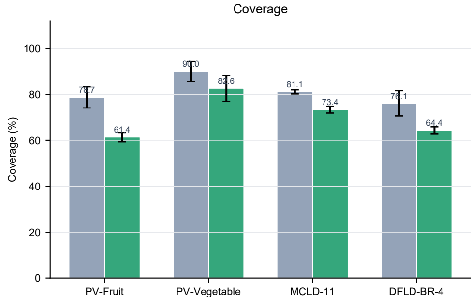
Parameter sensitivity at UMAP100: K=20 reference vs K=60 final configuration
