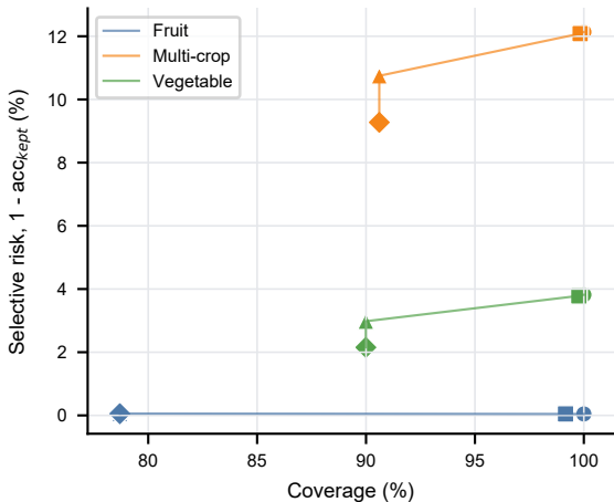
Discrete risk-coverage operating points
