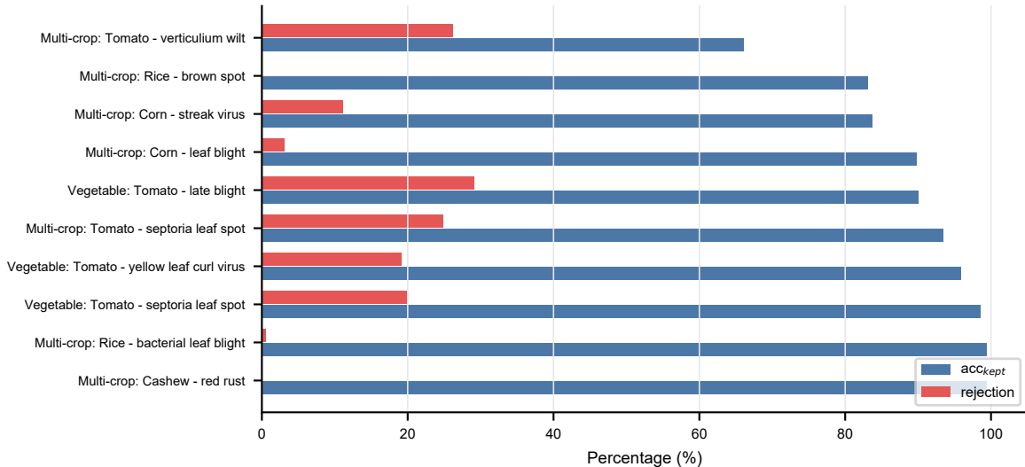
Class-level weak points across five seeds
