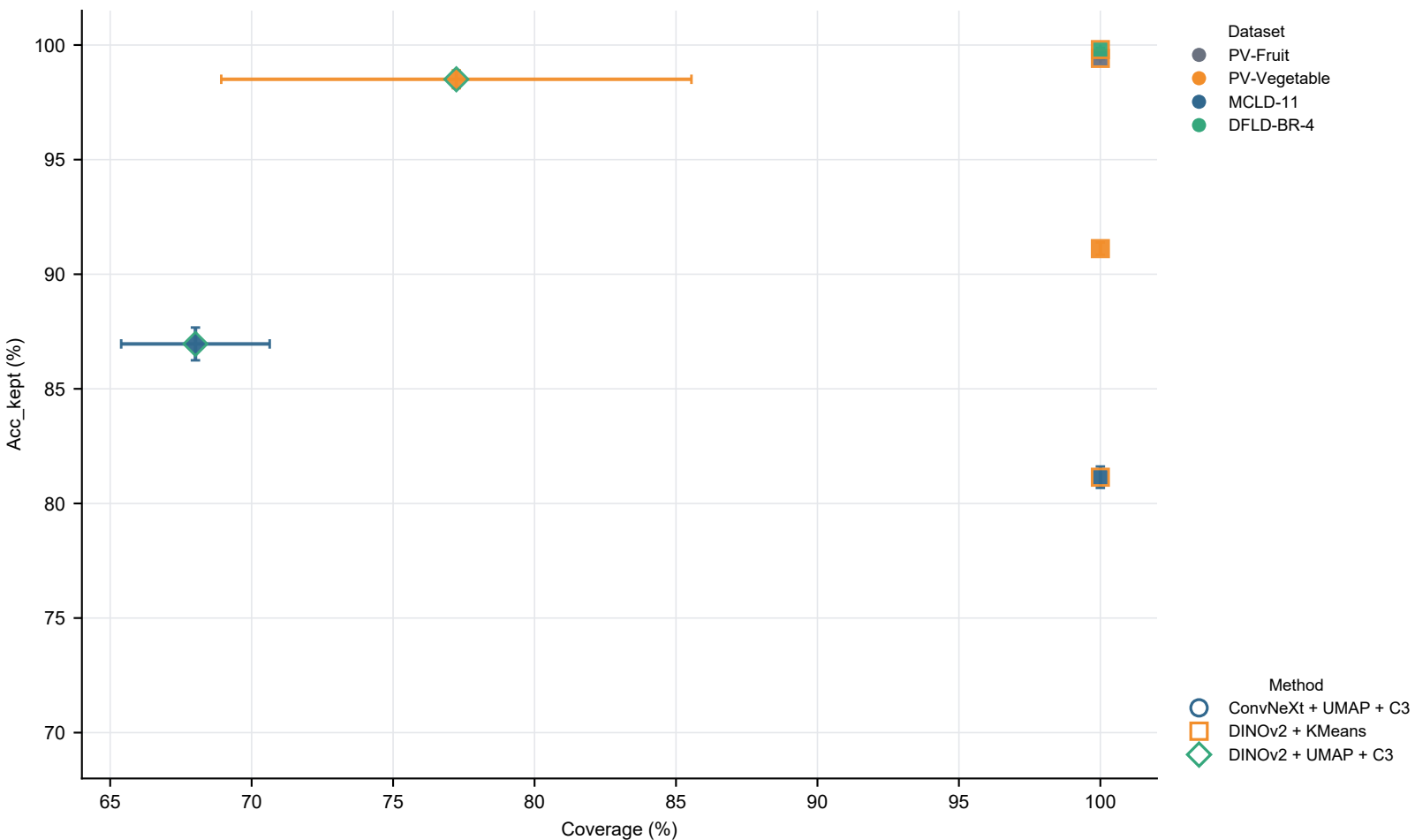
External DINOv2 baseline and cross-backbone validation
