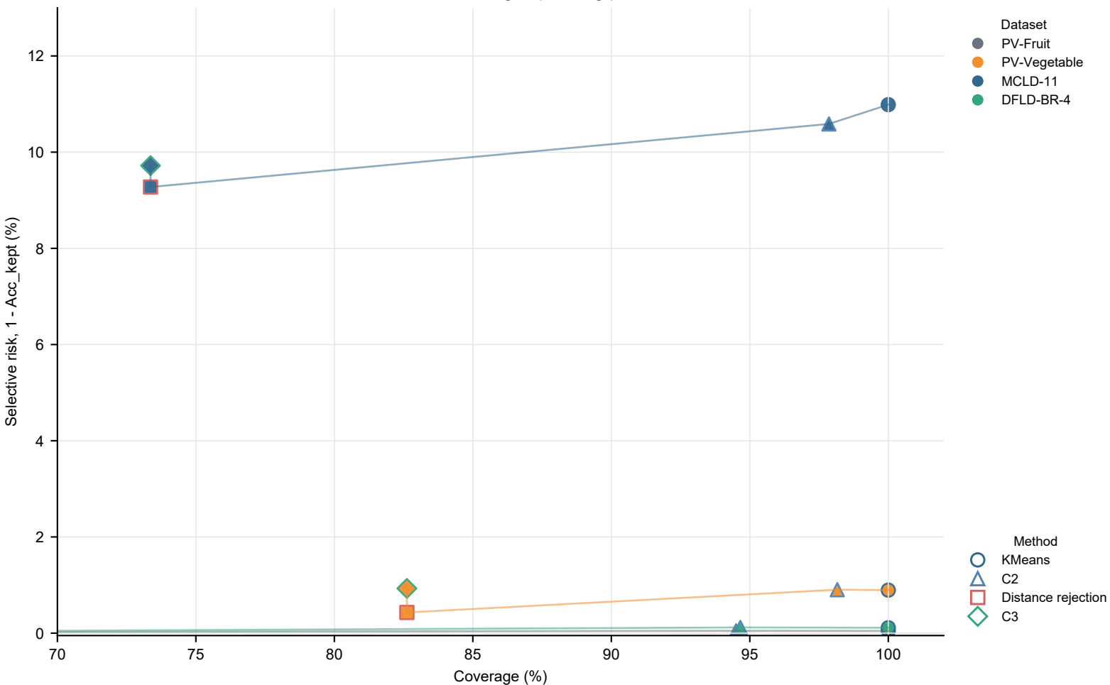
Discrete risk-coverage operating points
