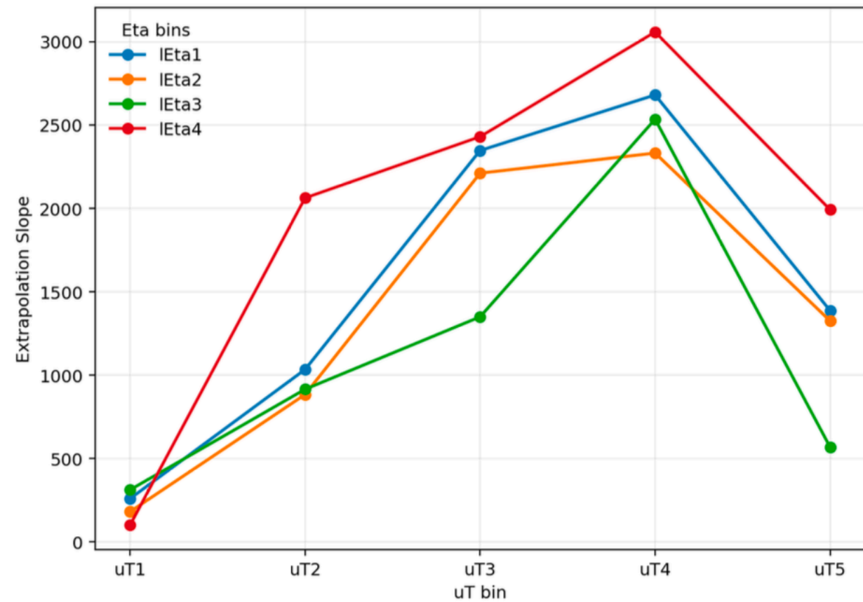
ptl extrapolation slopes vs uT (wplusenu_13TeV)
