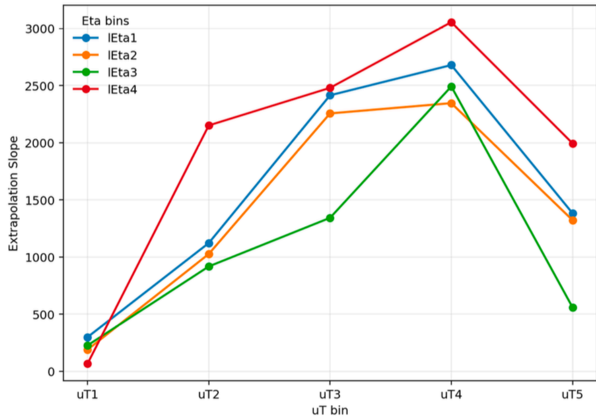
ptn extrapolation slopes vs uT (wplusenu_13TeV)
