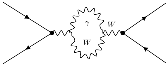
(f) W self-energy
