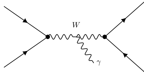
(c) W\gamma production
