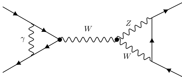
(e) Vertex correction
