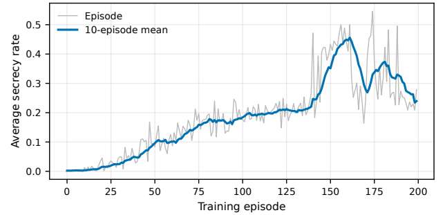
FIGURE 5 | Lightweight PPO diagnostic training curve from drl_ppo_200ep_5seed_stress_holdoutfit/training_log.csv . The smoothed curve shows the 10-episode moving average; the 200-episode run is not treated as a tuned DRL baseline.
