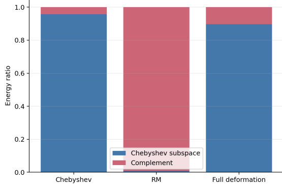
Fig. 7: Chebyshev projection leakage analysis. We project the Chebyshev branch, the RM branch, and the full deformation onto the predefined Chebyshev temporal subspace. Blue denotes the fraction of deformation energy explained by the Chebyshev subspace, while red denotes the fraction of energy lying in its complement. The RM branch is dominated by the complement component, indicating that it mainly captures residual deformation outside the low-order Chebyshev temporal subspace.
