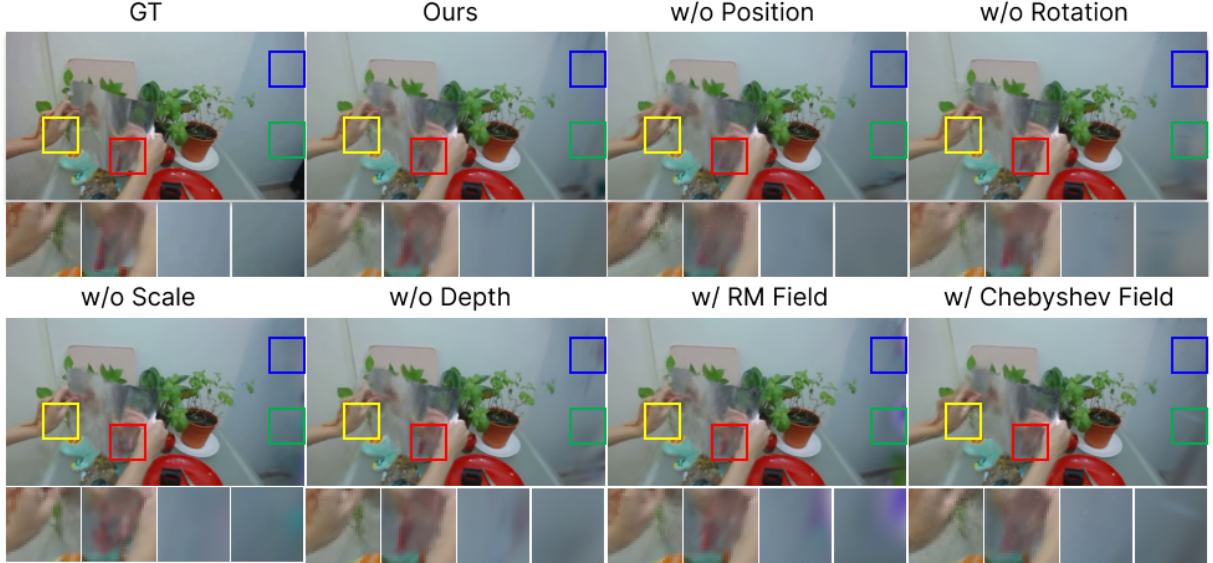
Fig. 6: Failure mode analysis of our method under component ablations. Visual comparison between the full framework and variants with individual components removed.
