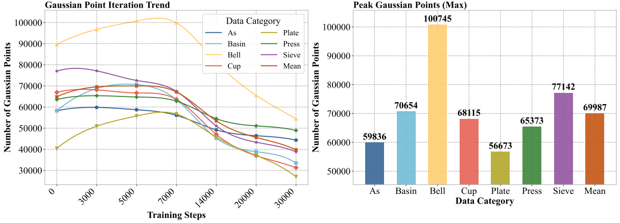
Fig. 3: Gaussian Point Change Analysis across Training. Evolution of the number of Gaussian points during training for different object categories (left), illustrating an initial expansion followed by category-dependent consolidation. The right panel reports the peak Gaussian count achieved for each category, revealing substantial variation in representation capacity requirements across object geometries. Objects with higher geometric complexity (e.g., Bell and Sieve) require significantly more Gaussian primitives, underscoring the necessity of deformation-field-based strategies rather than a uniform parameterization.
