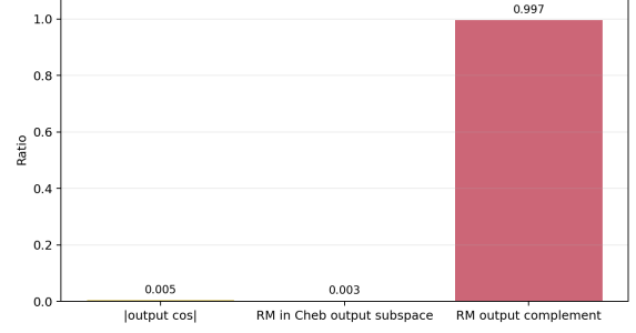
Fig. 8: Output-level orthogonality diagnostics. We measure the direct output overlap between the Chebyshev field and the RM field, and project the centered RM output onto the learned Chebyshev-output temporal subspace. The near-zero output overlap and low RM-to-Chebyshev-output leakage indicate that the RM branch has limited duplication of the Chebyshev output, while most RM energy remains in the complementary component.
