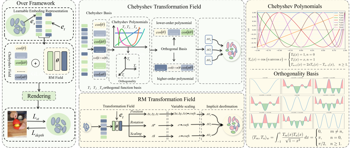
Fig. 1: Overview of the proposed framework. Our method adopts a divide-and-conquer strategy for monocular dynamic scene reconstruction by explicitly decomposing motion into two complementary transformation fields. The Chebyshev Transformation Field models globally coherent and temporally stable motion using a low-frequency spectral representation based on Chebyshev polynomial bases, providing a robust backbone for bounded, non-periodic motion. In parallel, the Residual Motion (RM) Field, implemented as a lightweight implicit model, captures localized and high-frequency motion components that lie outside the Chebyshev spectral subspace.
