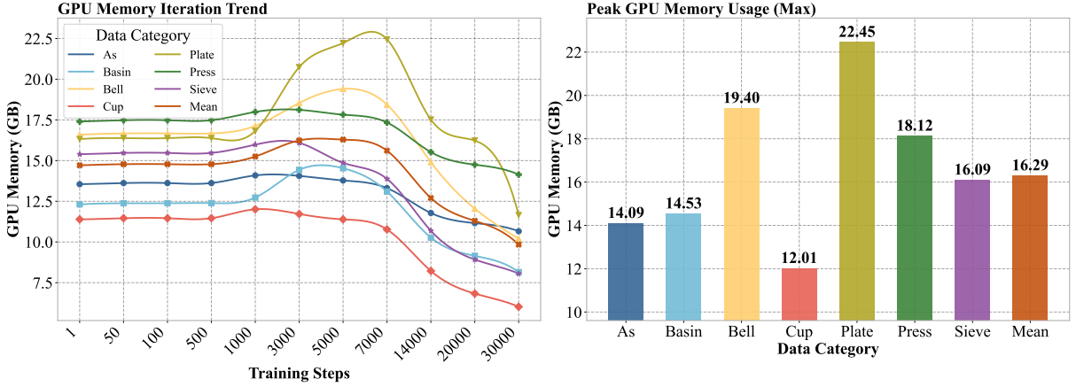
Fig. 4: GPU memory usage of the proposed method across scenes. Left: GPU memory consumption over training iterations. Right: Peak GPU memory usage during training.
