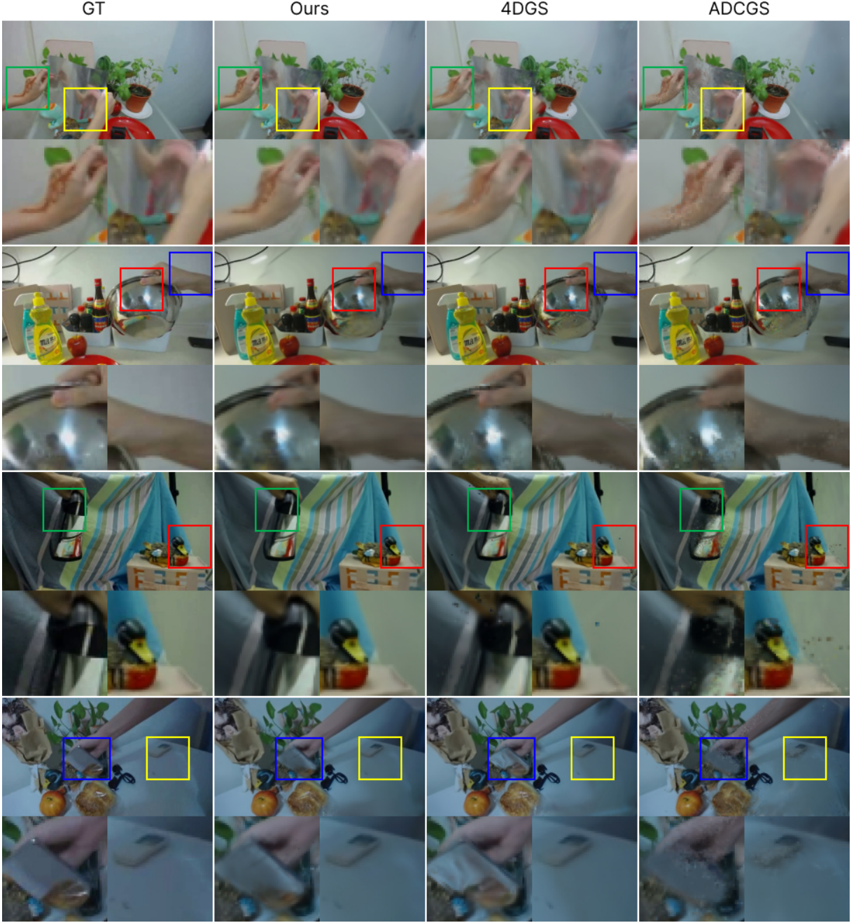
Fig. 5: Qualitative comparison with prior dynamic-scene methods demonstrates improved structural clarity and temporal consistency achieved by our approach.
