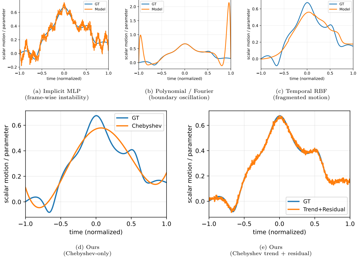
Fig. 2: Comparison of temporal modeling strategies on a representative 1D motion signal. (a) Implicit MLP-based modeling exhibits frame-wise instability and temporal jitter due to optimization conflicts. (b) Polynomial or Fourier-based representations suffer from boundary oscillations near temporal endpoints. (c) Temporal RBF modeling leads to fragmented motion with limited global coherence. (d) Chebyshev-only spectral modeling provides stable and smooth global motion trends but underfits localized variations. (e) Our full model combines a Chebyshev-based global trend with a residual motion component, achieving both temporal stability and accurate reconstruction of local dynamics.
