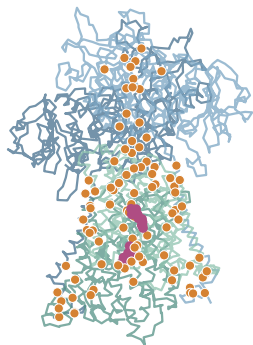
a 6LI9 assembly 1 · Ca traces
