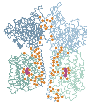
b Same assembly · rotated view
