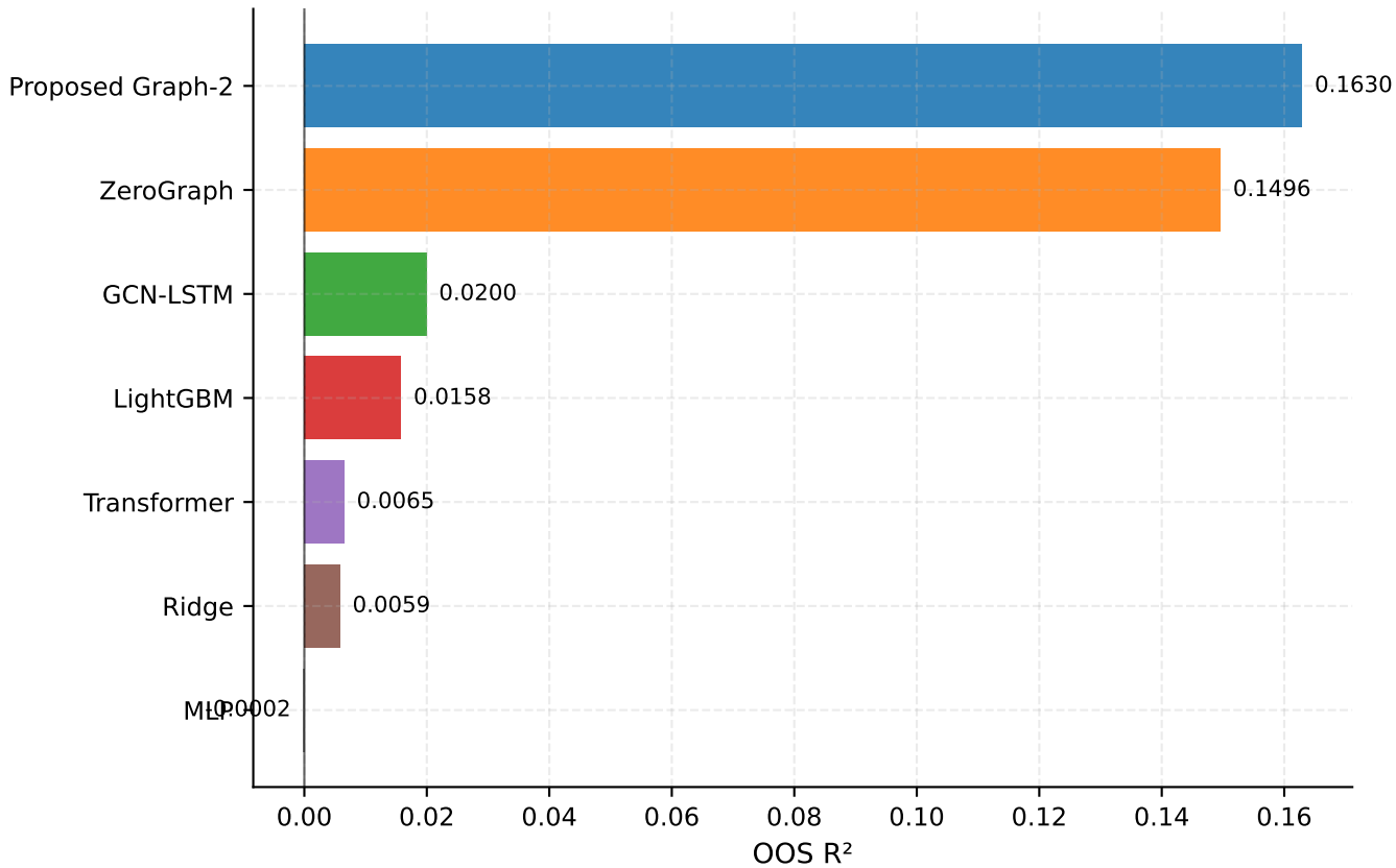
Overall out-of-sample R^2 by model
