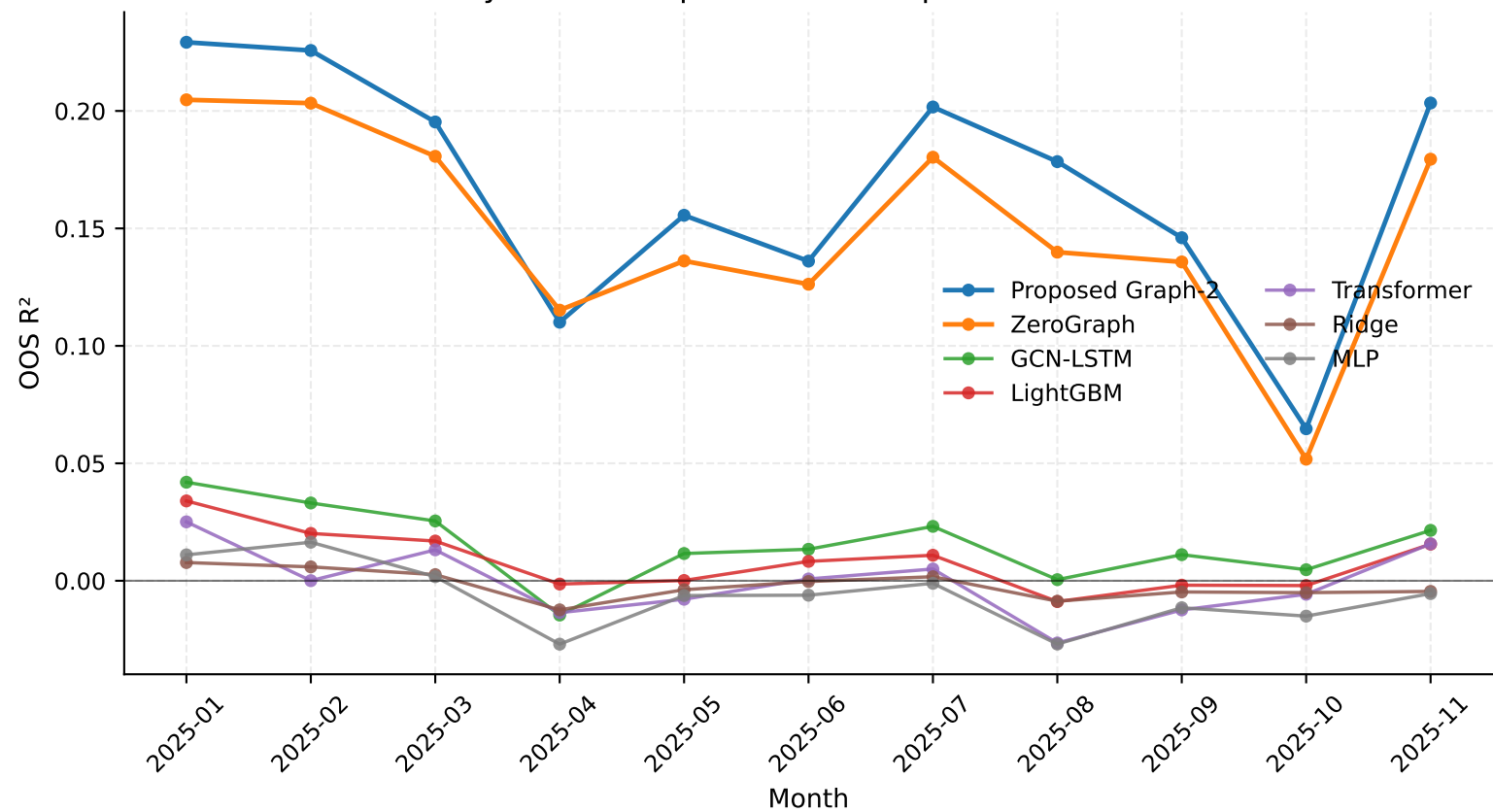
Monthly out-of-sample R^2 across representative models
