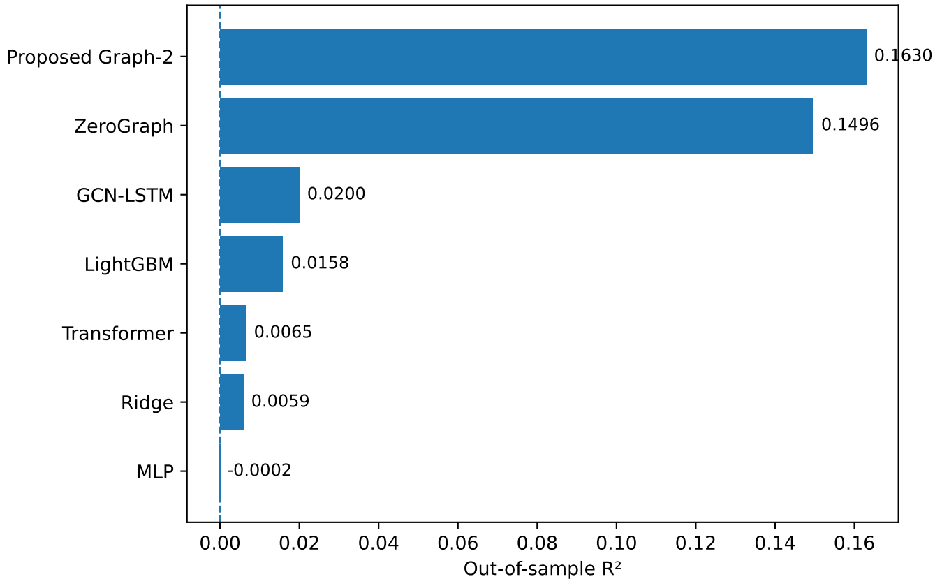
Out-of-sample R^2 comparison with representative benchmark models
