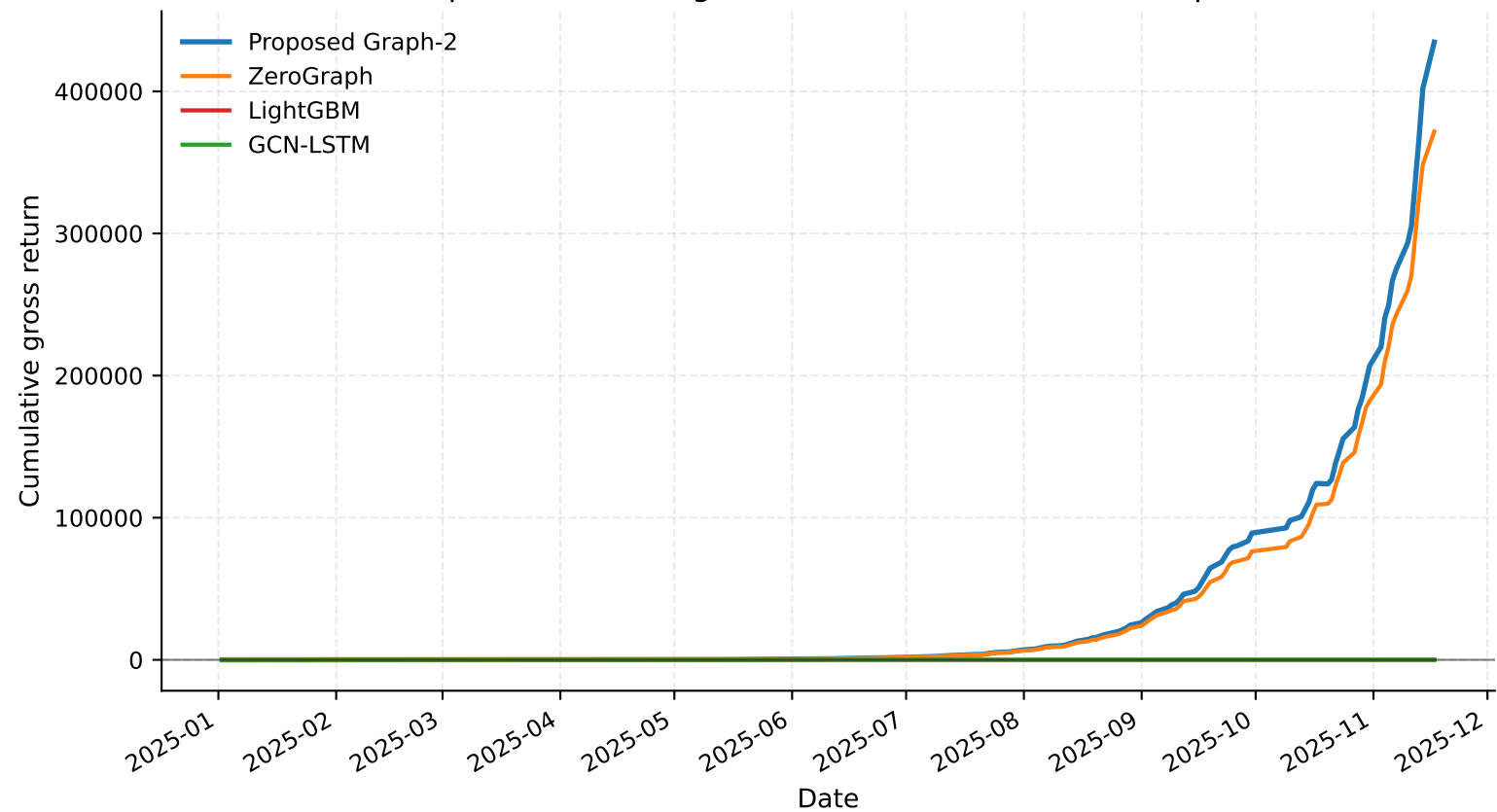
Top-5 cumulative gross return on the holdout sample
