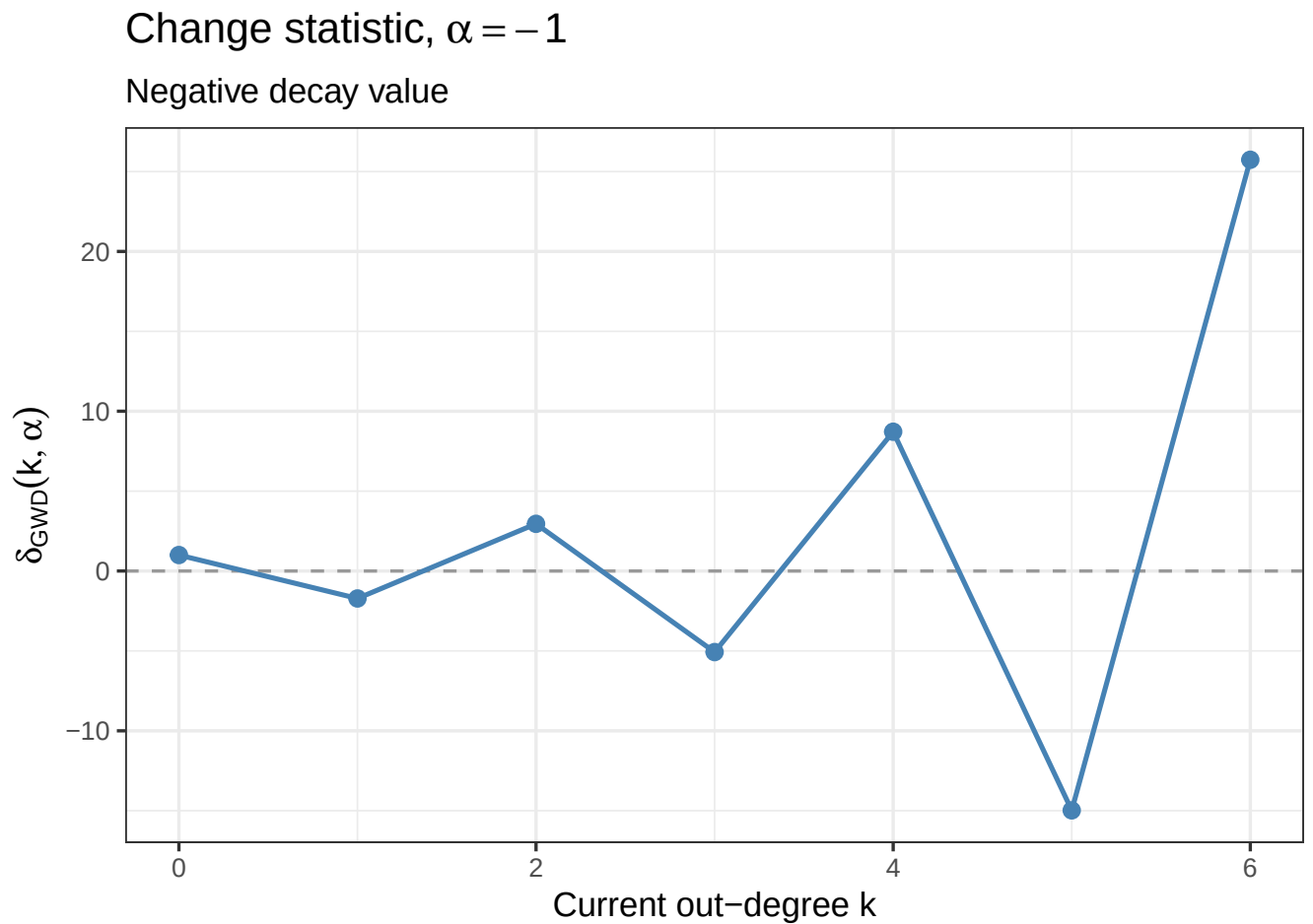
Figure 2: Change statistic for \alpha = -1 .
