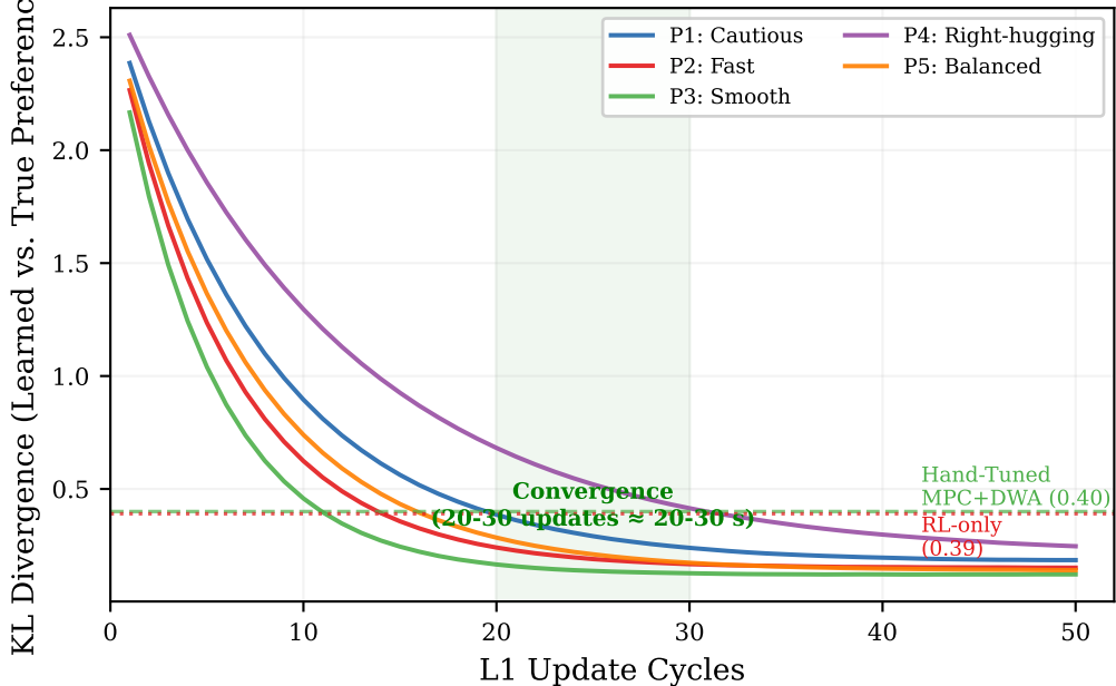
Figure 4: Preference learning convergence KL divergence vs. L1 updates, mean \pm 1\sigma over 50 runs
