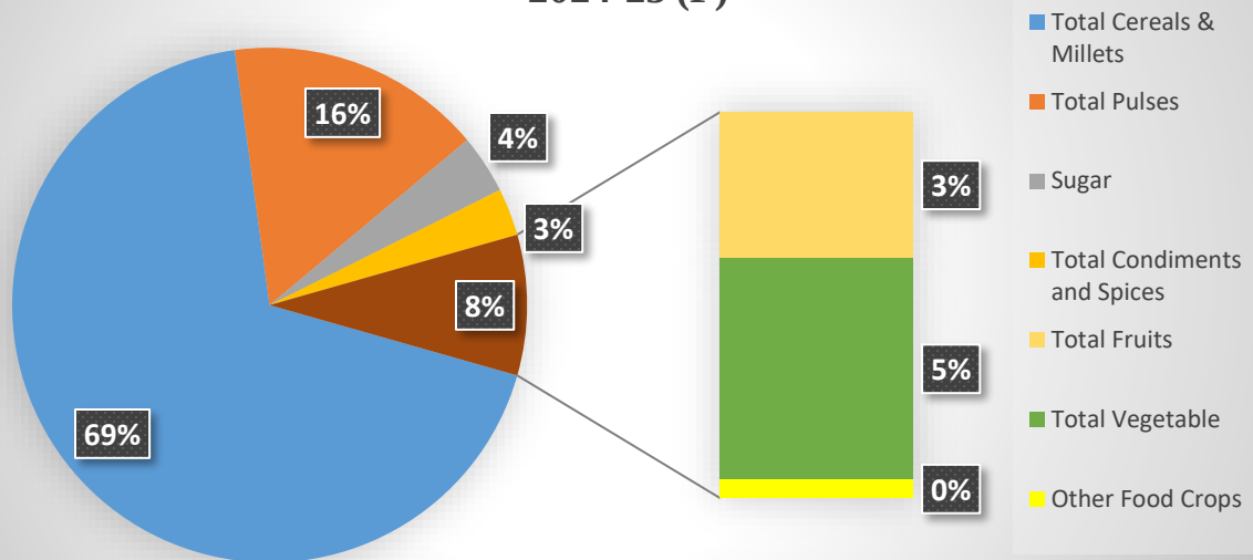
Figure 27: Composition of Area under Food Crops: 2024-25 (P)
