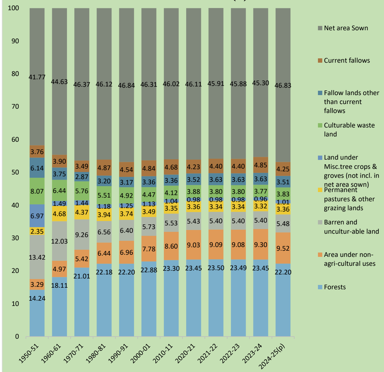
Figure 14: Transformation of India's Land Use Pattern over Seven Decades: Percentage Share Of Nine-fold Classification to Total Reported Area: 1950-51 to 2024-25(P)
