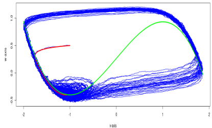
Trajectory of rough FHN system. Sigma = 0.03
