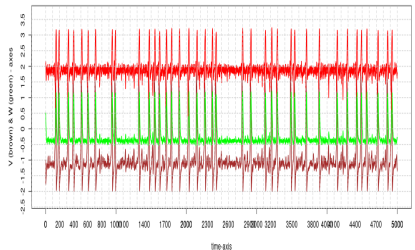
Time series rough FHN system
